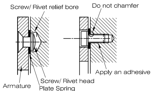
Armature type - 3 mounting dimensions
